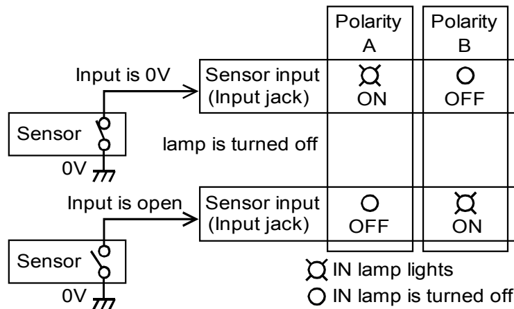
Input polarity and IN lamp
