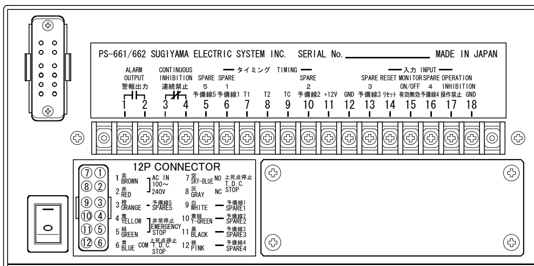
PS-661 back panel
