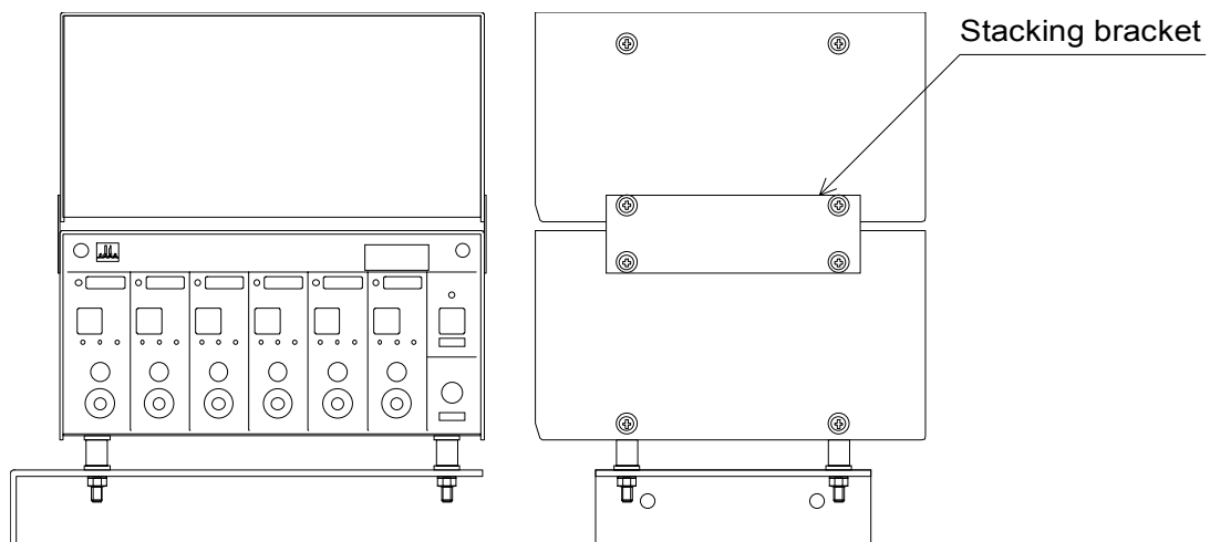
Installation with stacking bracket
