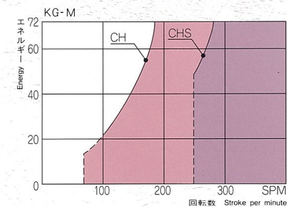
■回転数能力線図/ Energy graph
