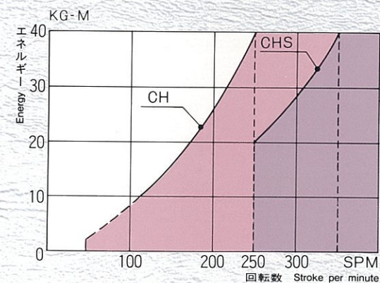
■回転数能力線図/ Energy graph
